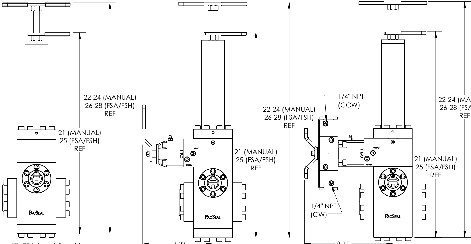
KR-75 Internal Override Remote Pilot Operation (-IO)
