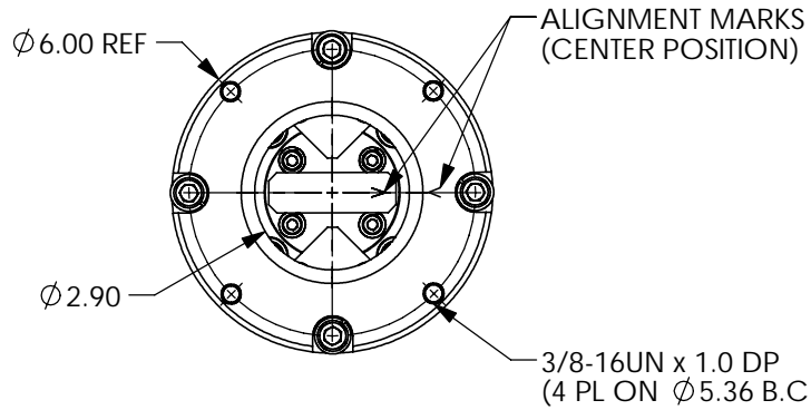
NEUTRAL POSITION
