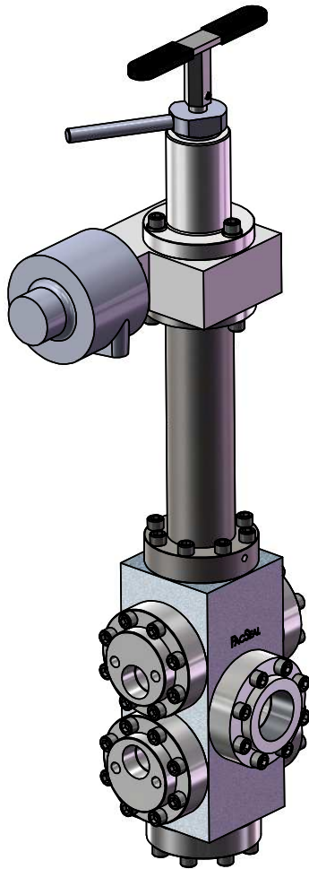
KR-150 Regulator with Failsafe Air Motor Operator
